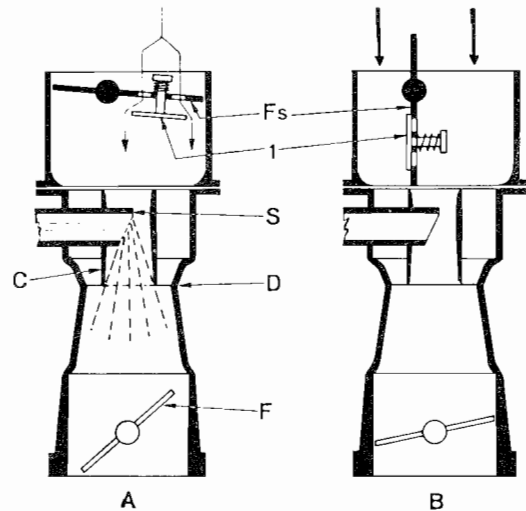
FIG. 16 Offset shutter with incorporated poppet valve type choke - 1 Anti-flooding poppet valve - Fs Shutter - S Spray nozzle - C Auxiliary (or secondary) Venturi - D Main (or primary) Venturi - F Throttle valve - A Choke in operation - B Choke excluded.
