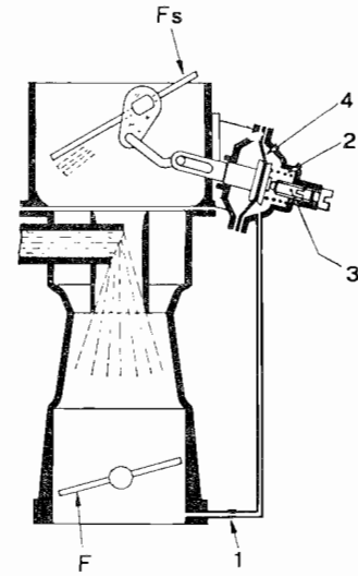
FIG. 15 Pneumatic overchoking or antiflooding device - 1 Limiter jet on vacuum channel - 2 Diaphragm return spring - 3 Adjusting screws - 4 Diaphragm - Fs Choke valve - F Throttle valve.
