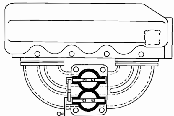
FIG. 47-B Dual-barrel, downdraft carburetor with synchronized opening of throttles , installed on an in-line engine. For maximum power each carburetor barrel feeds only two cylinders and the manifold does not have a common chamber under the carburetor.
